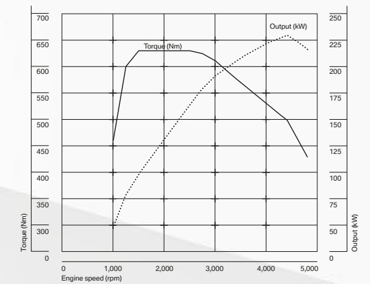
Peak torque of 630Nm is on tap between 1,500 and 2,500rpm. As a result, the BMW 535d reacts with impressive force to even light pressure on the accelerator pedal.
