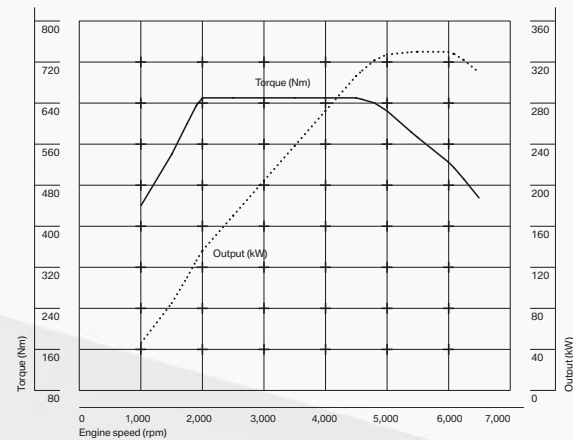
Impressive performance: the BMW TwinPower Turbo eight-cylinder petrol engine in the BMW 5 Series Gran Turismo 550i.
